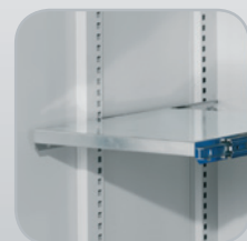
Pull-out shelf 500 galvanized, full extension. Makes handling of heavy items easier
