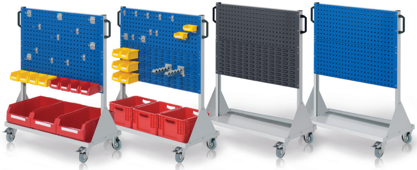
RasterMobil® Size 3 - H 1230 x W 1000 x D 500 mm
