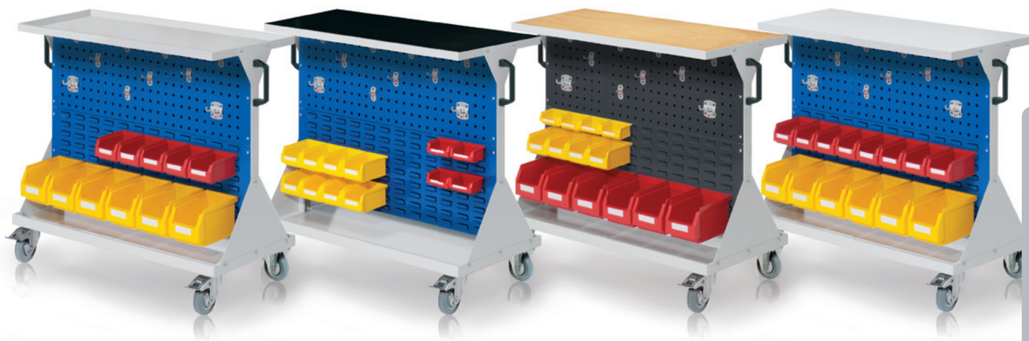
RasterMobil® Size 2 - H 930 x W 1000 x D 500 mm
