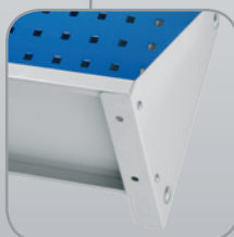
*RasterPlan movable walls are equipped with hidden fixing holes for floor anchoring.
