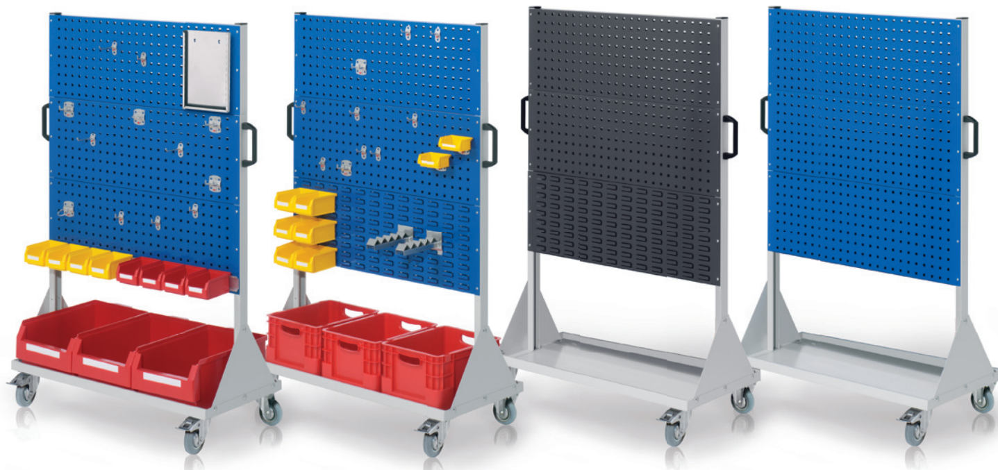
RasterMobil® Size 4 - H 1580 x W 1000 x D 500 mm
